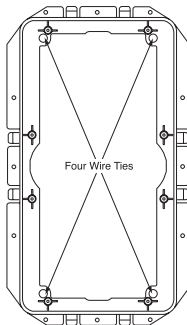
Figure 11. The brackets have four wire-tie points.
